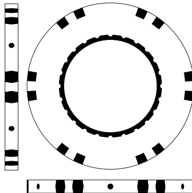
6 SMALL INSERT 5.94.013
