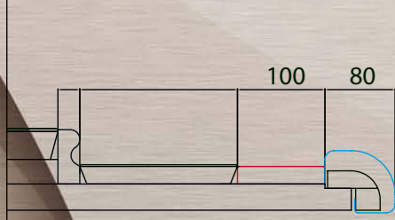
2 levels table 100 mm Wood / 80 mm Upholstery
