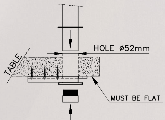
INTERNAL TABLE MOUNTING
