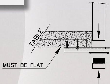
EXTERNAL TABLE MOUNTING
