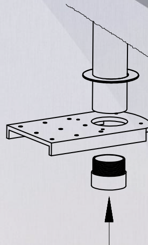
EXTERNAL TABLE MOUNTING
